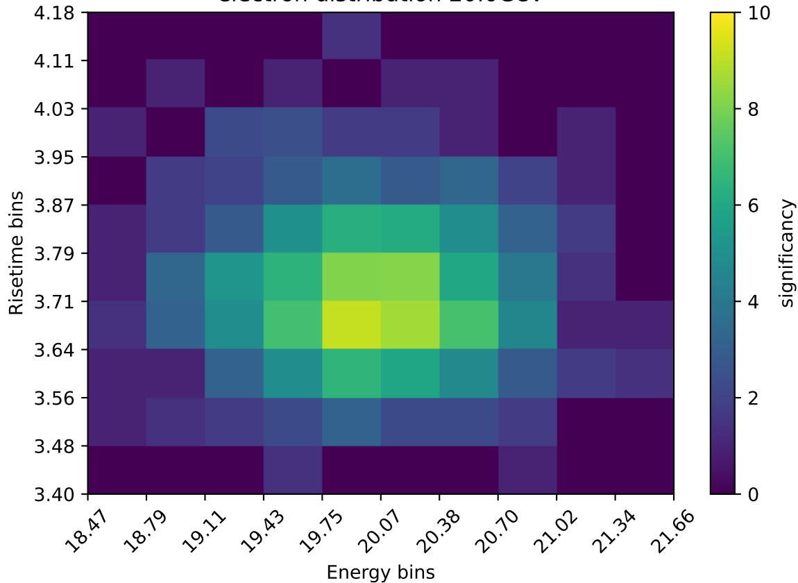
electron distribution 20.0GeV
